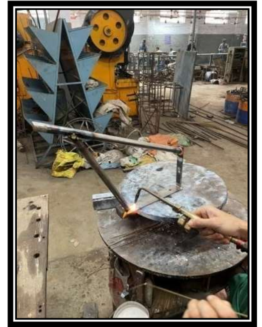
GAS WELDING
