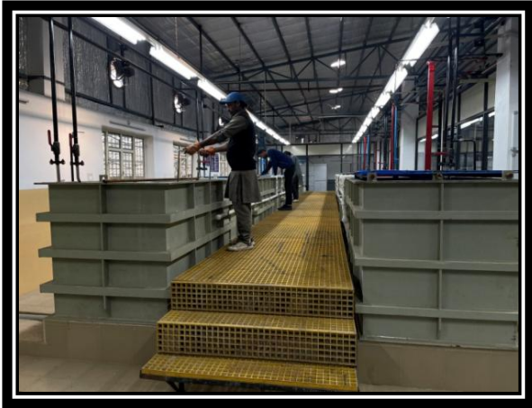
7 TANK PHOSPHATING AND ELECTROPLATING WITH TEMPERATURE CONTROL
