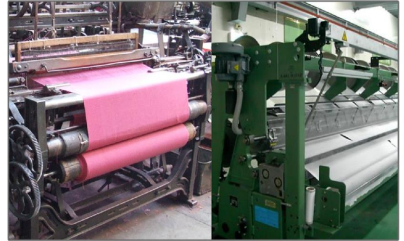
Weaving process
