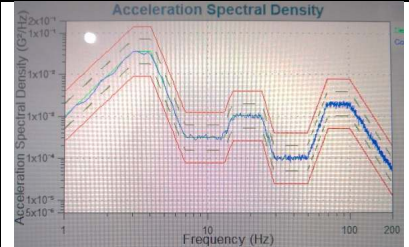
Block 12 Face 3 Test Vibration Profile
