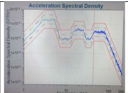
Block 12 Face 6 Test Vibration Profile
